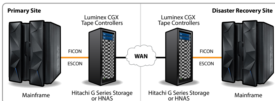
Typical CGX-Hitachi Disaster Recovery configuration using replication over a WAN
